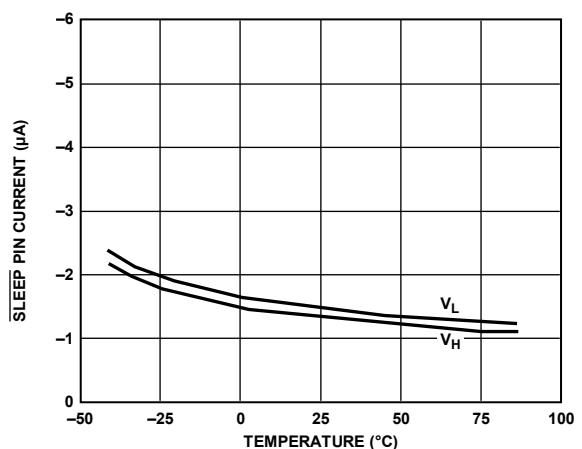
Figure 8. SLEEP Pin Current vs. Temperature
