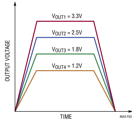
Figure 3. Output Ratiometric Tracking Waveform
