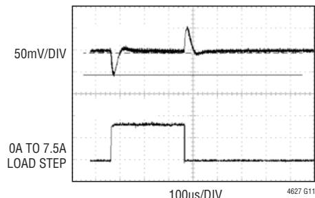
3.3V Transient Response
