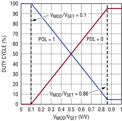
LTC6992-3
