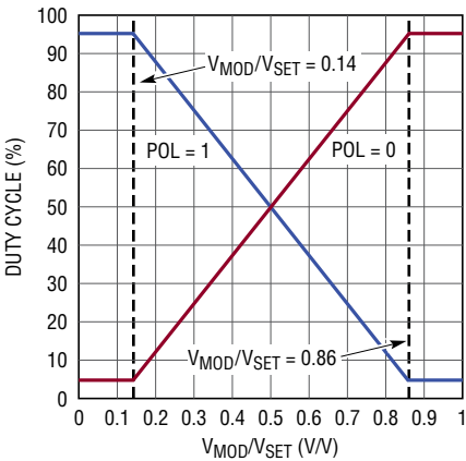
LTC6992-2
