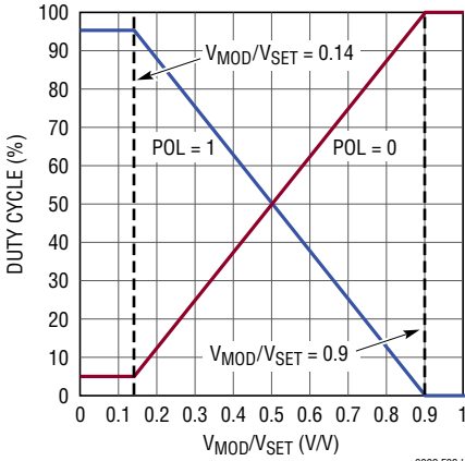
LTC6992-4
