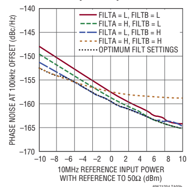
Additive Phase Noise vs Input Amplitude
