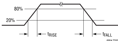
Differential LVPECL Rise/Fall Times
