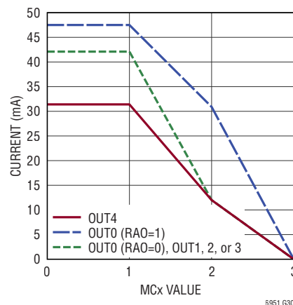
V_{\text{OUT}}^+ Supply Current per Output vs MCx Value
