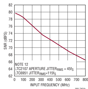
SNR vs Input Frequency of LTC6951 Clocking an LTC2107, f_s = 210\text{MSPS} , A_{IN} = -3\text{dBFS}
