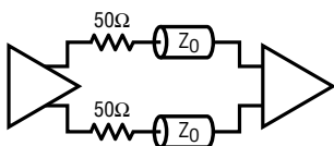
NEAR END TERMINATION (SERIES TERMINATION)
