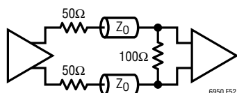
NEAR AND FAR END TERMINATION (DOUBLE TERMINATION)
