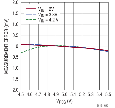
Measurement Error vs V_{\text{REG}}
