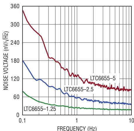
Figure 19. LTC6655-2.5 Low Frequency Noise Spectrum
