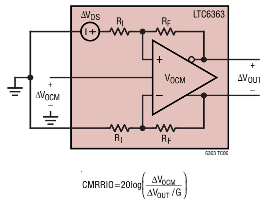
Figure 11. Specified LTC6363-0.5, LTC6363-1 and LTC6363-2 CMRR10 Is Referred to the Input Pins of the Part
