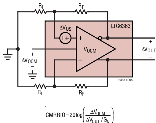
Figure 10. Specified LTC6363 CMRR10 Is Referred to the Summing Junction
