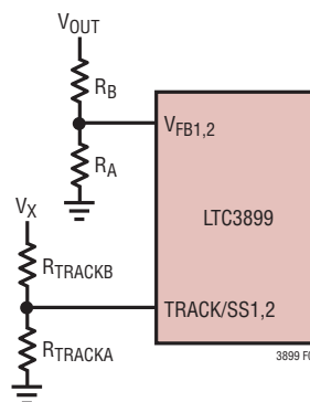
Figure 7. Two Different Modes of Output Voltage Tracking
