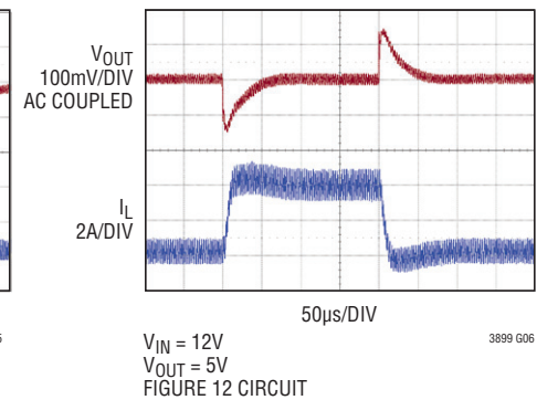
Load Step (Buck) Forced Continuous Mode
