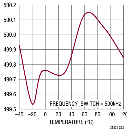
PWM Frequency vs Temperature
