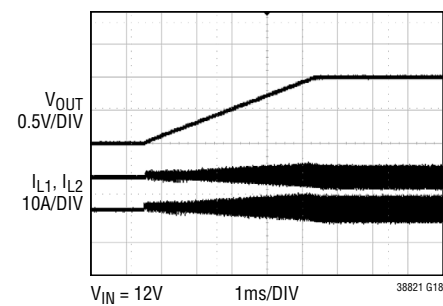
Soft-Start Ramp
