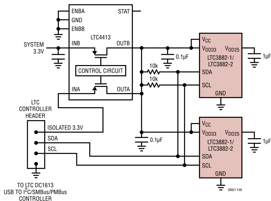
Figure 48. DC1613 Connections (V DD33 Supply)
