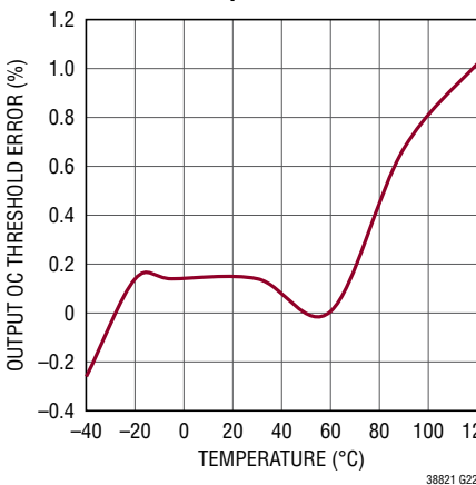
Output Overcurrent Threshold Error vs Temperature
