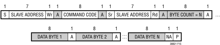
Figure 15. Block Read Protocol
