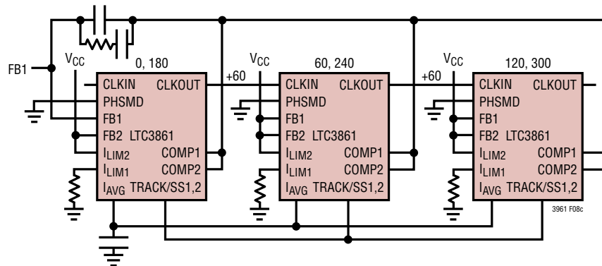
Figure 8c. 6-Phase Operation
