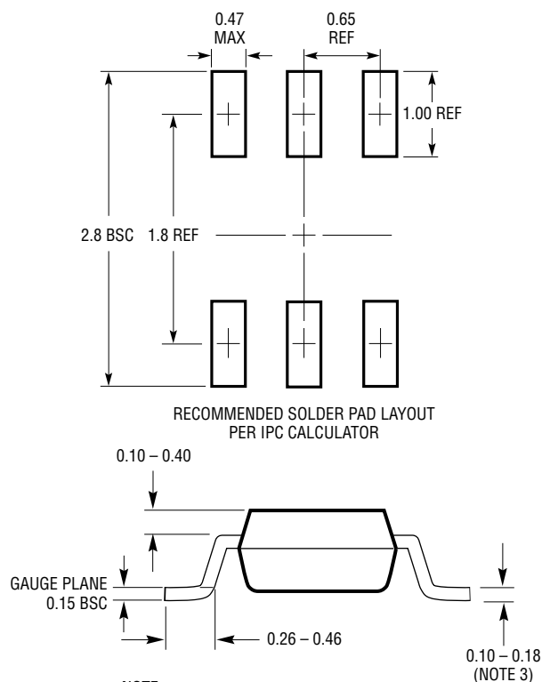
SC6 Package 6-Lead Plastic SC70 (Reference LTC DWG # 05-08-1638 Rev B)
