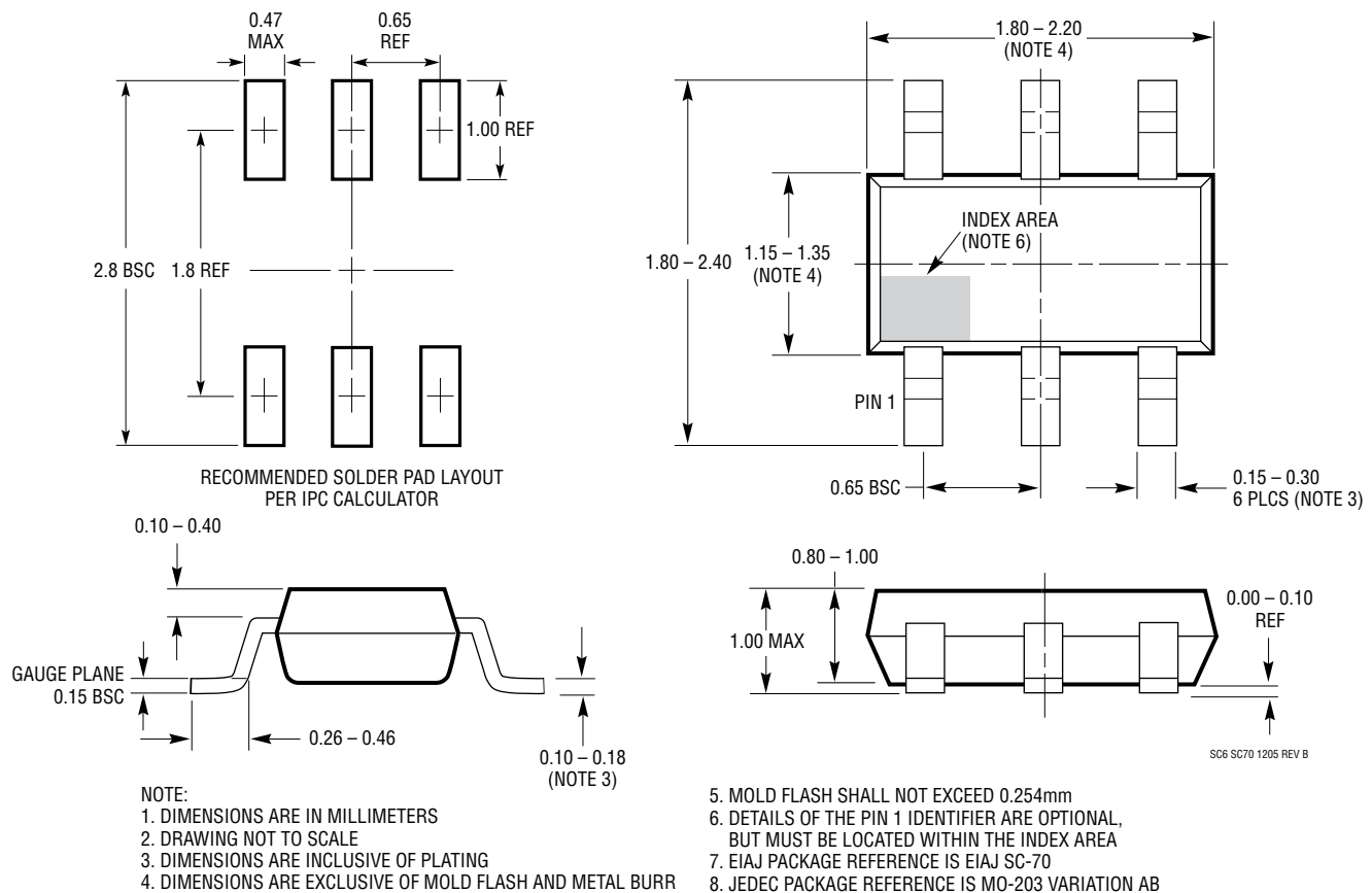
SC6 Package 6-Lead Plastic SC70 (Reference LTC DWG # 05-08-1638 Rev B)
