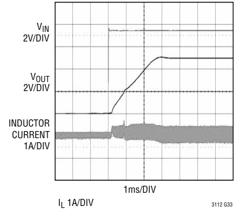
7.5V IN to 5.0V OUT Soft-Start Waveforms
