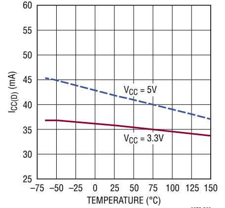
Supply Current (Dominant) vs Temperature
