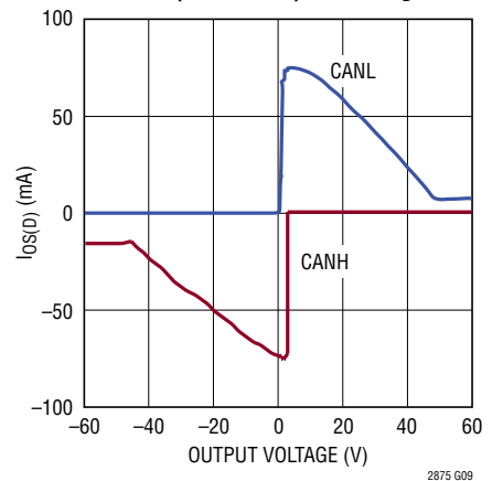
Driver Output Short-Circuit Current (Dominant) vs Voltage
