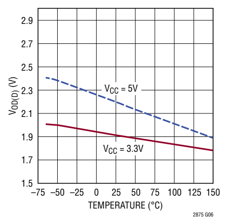
Driver Differential Output Voltage (Dominant) vs Temperature
