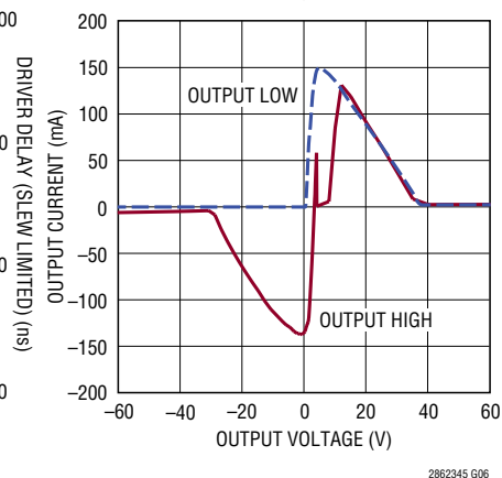
Driver Output Short-Circuit Current vs Voltage
