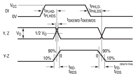
Figure 4. Driver Timing Measurement
