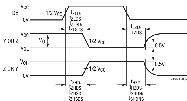
Figure 5. Driver Enable and Disable Timing Measurement
