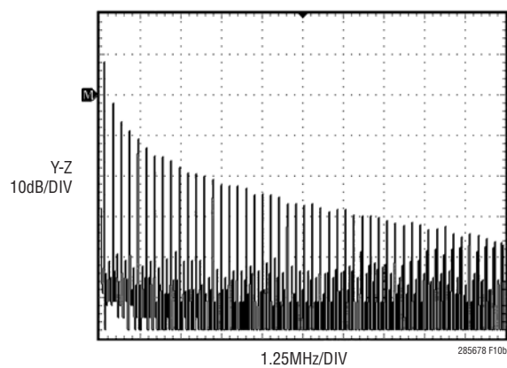
Figure 10. LTC2858-1 Driver Output at 100kHz Into 100Ω Resistor
