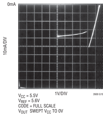
Short-Circuit Output Current vs V_{OUT} (Sourcing)
