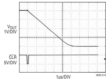
Hardware \overline{CLR}
