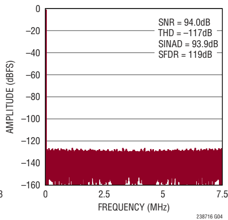
32k Point FFT f_{SAMPL} = 15\text{Mpsps} , f_{IN} = 2\text{kHz}
