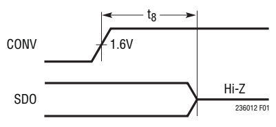
Figure 1. SDO Into Hi-Z State After CONV Rising Edge
