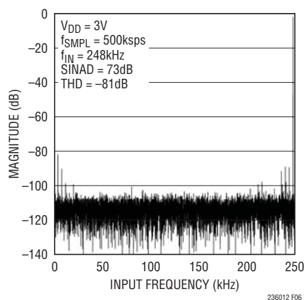
Figure 6. LTC2362 FFT Plot
