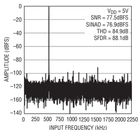
32k Point FFT, f_S = 4.5\text{Mps} , f_{IN} = 500\text{kHz}
