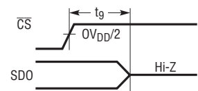
Figure 2. SDO Into Hi-Z after CS↑
