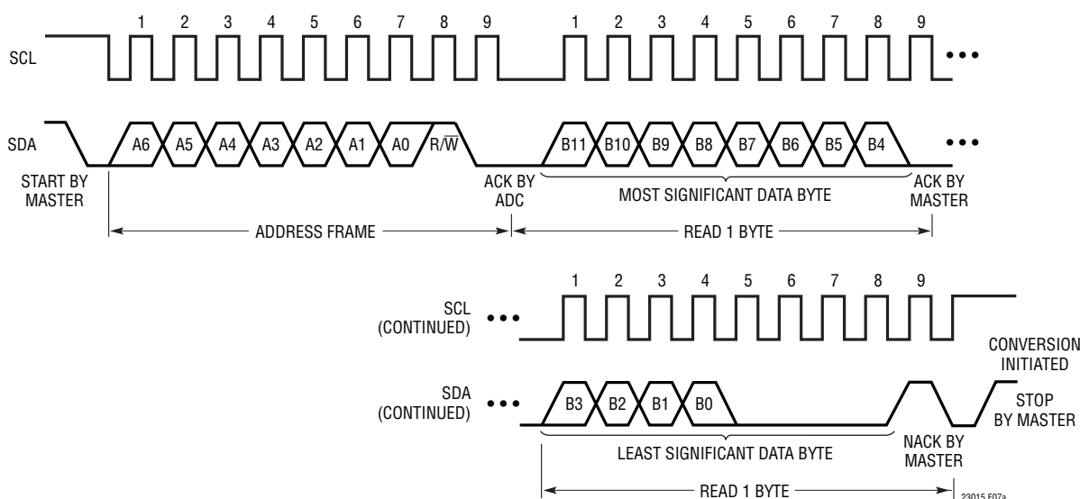
Figure 7a. Timing Diagram for Reading from the LTC2301/LTC2305
