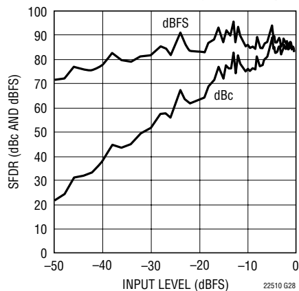
LTC2250: SFDR vs Input Level, f_{IN} = 70\text{MHz} , 2V Range, 105Mps
