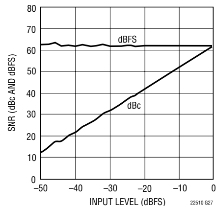
LTC2250: SNR vs Input Level, f_{IN} = 70\text{MHz} , 2V Range, 105Mps
