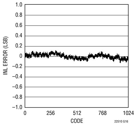
LTC2250: Typical INL, 2V Range, 105Mps
