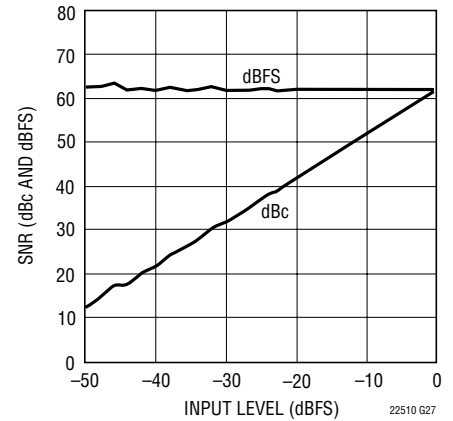
LTC2250: SNR vs Input Level, f_{IN} = 70\text{MHz} , 2V Range, 105Msps
