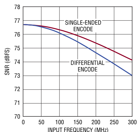
LTC2184: SNR vs Input Frequency, -1\text{dBFS} , 105\text{Mps} , 2\text{V} Range
