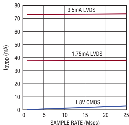
LTC2182: I_{OVPD} vs Sample Rate, 5\text{MHz} , -1\text{dBFS} , Sine Wave Input on Each Channel
