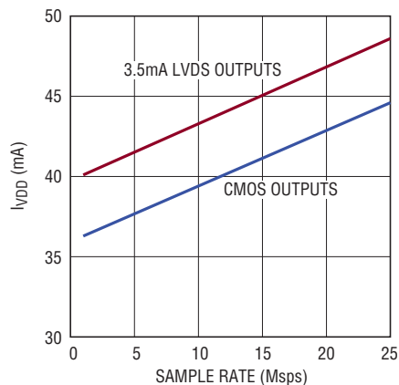
LTC2182: I_{VDD} vs Sample Rate, 5\text{MHz} , -1\text{dBFS} , Sine Wave Input on Each Channel
