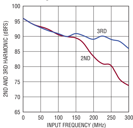
LTC2182: 2nd, 3rd Harmonic vs Input Frequency, -1\text{dBFS} , 25\text{Mpsps} , 1\text{V} Range
