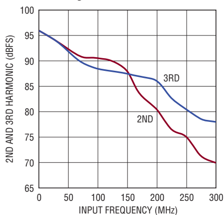
LTC2182: 2nd, 3rd Harmonic vs Input Frequency, -1\text{dBFS} , 25\text{Mpsps} , 2\text{V} Range
