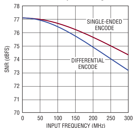
LTC2182: SNR vs Input Frequency, -1\text{dBFS} , 25\text{Mpsps} , 2\text{V} Range
