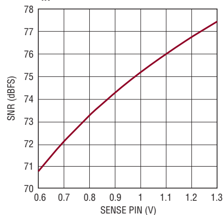
LTC2182: SNR vs SENSE, f_{IN} = 5\text{MHz} , -1\text{dBFS}
