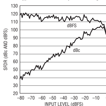
LTC2182: SFDR vs Input Level, f_{IN} = 70\text{MHz} , 25\text{Mpsps} , 2\text{V} Range
