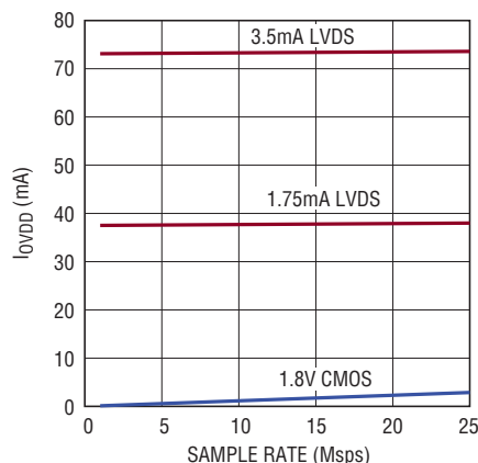
LTC2181: I_{OVPD} vs Sample Rate, 5\text{MHz} , -1\text{dBFS} , Sine Wave Input on Each Channel
