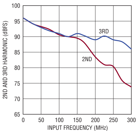
LTC2182: 2nd, 3rd Harmonic vs Input Frequency, -1dBFS, 65Mps, 1V Range
