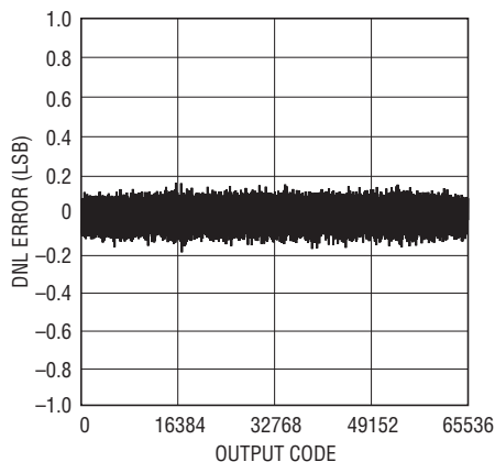
LTC2181: Differential Non-Linearity (DNL)
