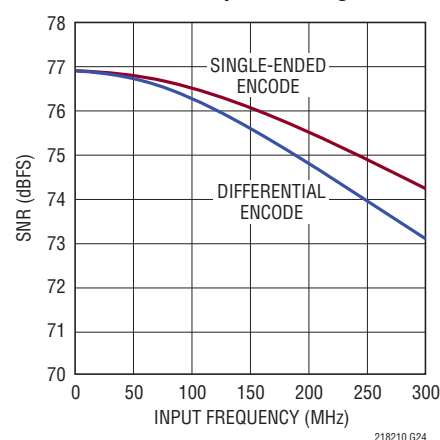
LTC2181: SNR vs Input Frequency, -1\text{dBFS} , 40\text{Mps} , 2\text{V} Range
