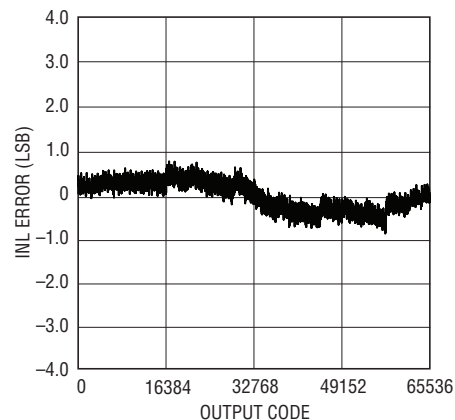
LTC2181: Integral Non-Linearity (INL)
