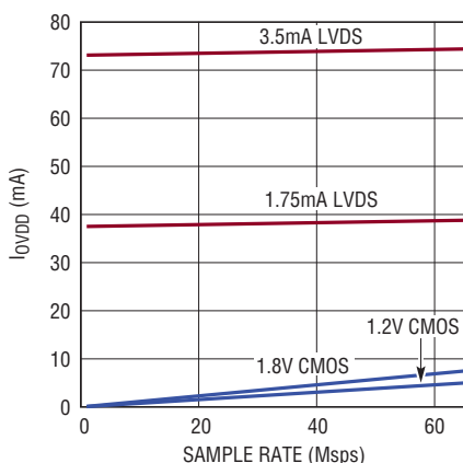
LTC2182: I_{OVPD} vs Sample Rate, 5MHz, -1dBFS, Sine Wave Input on Each Channel
