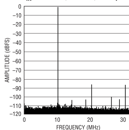
LTC2182: 64k Point FFT, f_{IN} = 140\text{MHz} , -1dBFS, 65Msps
