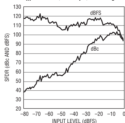
LTC2181: SFDR vs Input Level, f_{IN} = 70\text{MHz} , 40\text{Mps} , 2\text{V} Range
