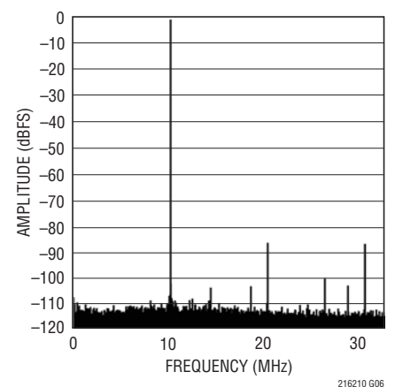
LTC2162: 64k Point FFT, f_{IN} = 140\text{MHz} , -1\text{dBFS} , 65\text{Mpsps}
