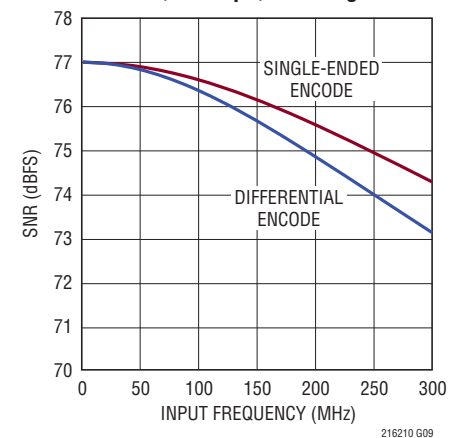
LTC2162: SNR vs Input Frequency, -1\text{dBFS} , 65\text{Mpsps} , 2\text{V} Range
