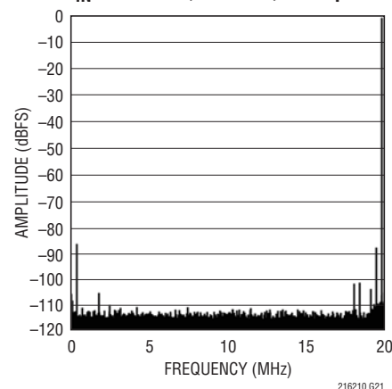
LTC2161: 64k Point FFT, f_{IN} = 140\text{MHz} , -1\text{dBFS} , 40\text{Mps}
