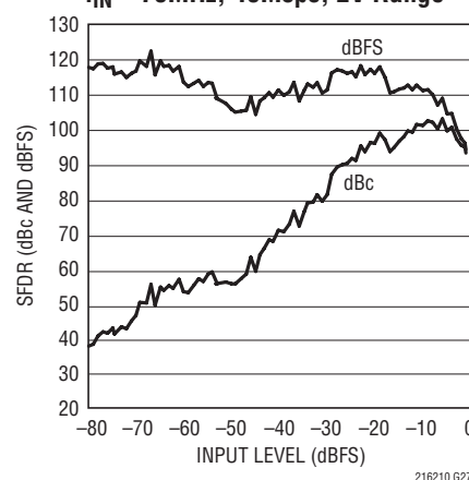
LTC2161: SFDR vs Input Level, f_{IN} = 70\text{MHz} , 40\text{Mps} , 2\text{V} Range
