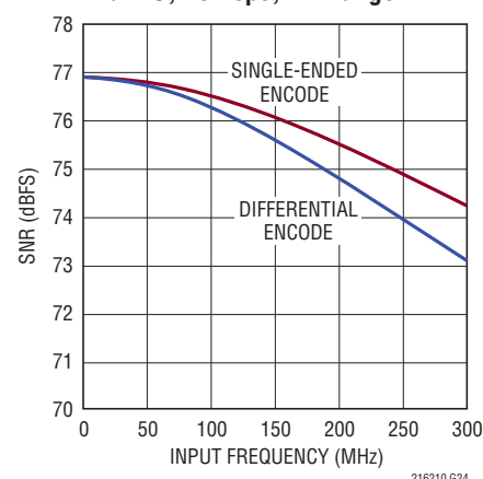
LTC2161: SNR vs Input Frequency, -1\text{dBFS} , 40\text{Mps} , 2\text{V} Range
