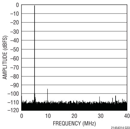
LTC2143-14: 64k Point FFT, f_{IN} = 5MHz , -1dBFS, 80MSPS
