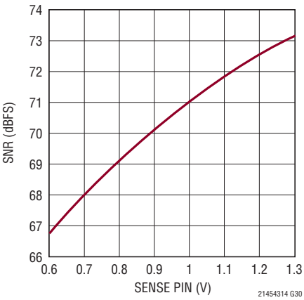
LTC2144-14: SNR vs SENSE, f_{IN} = 5MHz , -1dBFS
