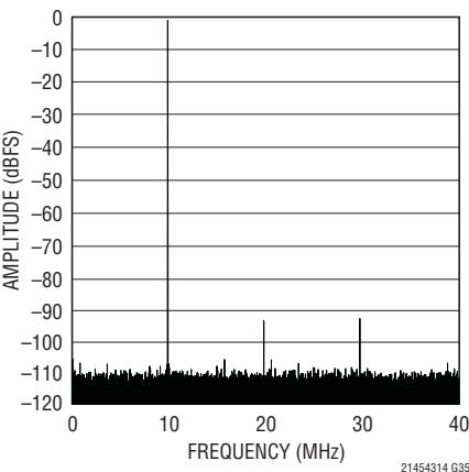
LTC2143-14: 64k Point FFT, f_{IN} = 70MHz , -1dBFS, 80MSPS
