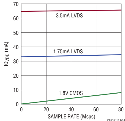
LTC2143-14: I_{O_VDD} vs Sample Rate, 5\text{MHz} , -1\text{dBFS} , Sine Wave Input on Each Channel
