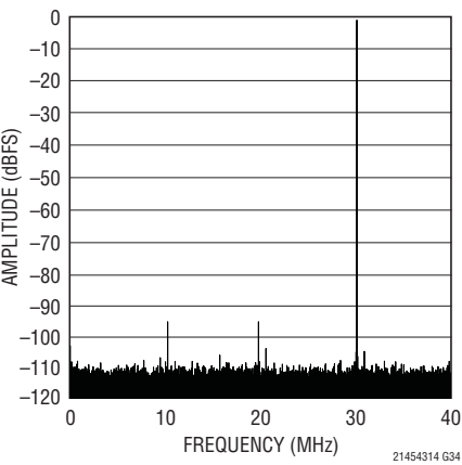
LTC2143-14: 64k Point FFT, f_{IN} = 30MHz , -1dBFS, 80MSPS
