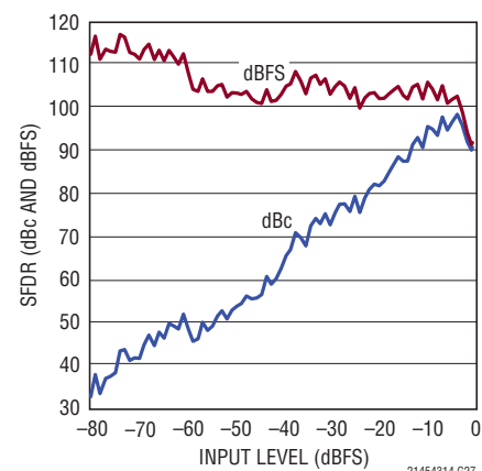
LTC2144-14: SFDR vs Input Level, f_{IN} = 70\text{MHz} , 105\text{Mps} , 2\text{V} Range
