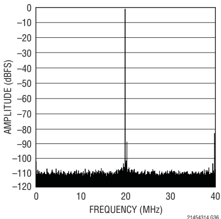
LTC2143-14: 64k Point FFT, f_{IN} = 140MHz , -1dBFS, 80MSPS
