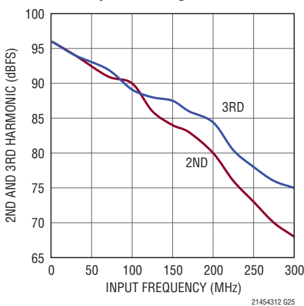
LTC2144-12: 2nd, 3rd Harmonic vs Input Frequency, -1\text{dBFS} , 105\text{Mps} , 2\text{V} Range
