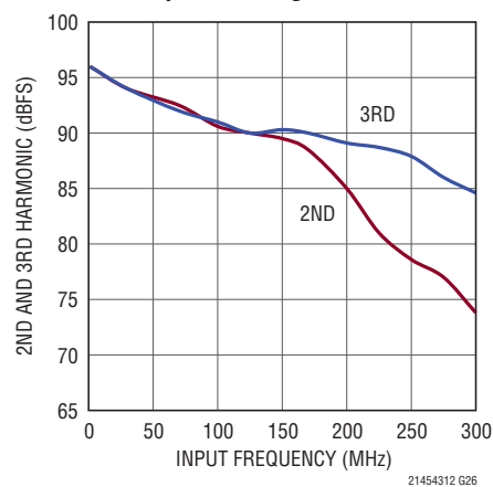
LTC2144-12: 2nd, 3rd Harmonic vs Input Frequency, -1\text{dBFS} , 105\text{Mps} , 1\text{V} Range
