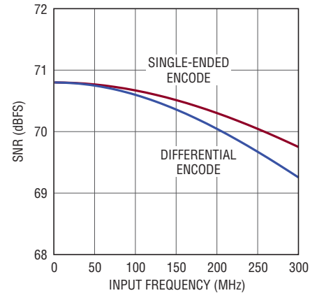
LTC2143-12: SNR vs Input Frequency, -1\text{dBFS}, 80\text{Mps}, 2V Range
