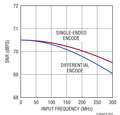
LTC2144-12: SNR vs Input Frequency, -1\text{dBFS} , 105\text{Mps} , 2\text{V} Range
