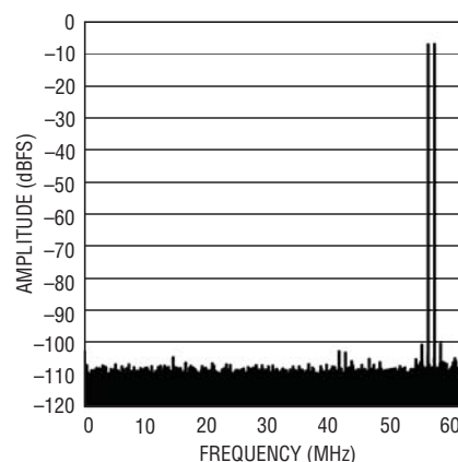
2-Tone FFT, f_{IN} = 70MHz and 69MHz
