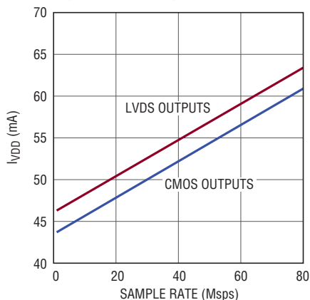
LTC2143-12: I_{VDD} vs Sample Rate, 5MHz, -1\text{dBFS} Sine Wave Input on Each Input
