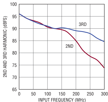
LTC2143-12: 2nd, 3rd Harmonic vs Input Frequency, -1\text{dBFS}, 80\text{Mps}, 1V Range
