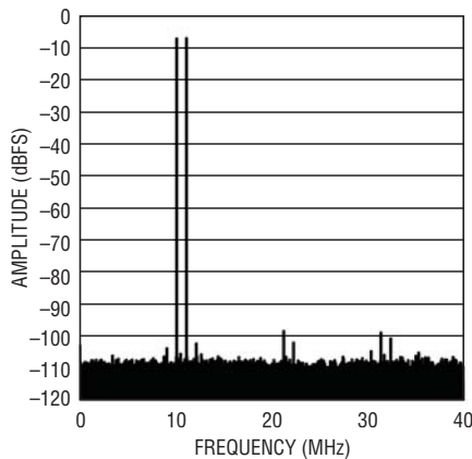
LTC2143-12: 64k Point 2-Tone FFT, f_{IN} = 69\text{MHz}, 70\text{MHz}, -7\text{dBFS}, 80Mps
