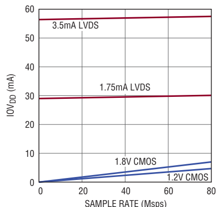
LTC2143-12: I_{O VDD} vs Sample Rate, 5MHz, -1\text{dBFS} , Sine Wave on Each Channel
