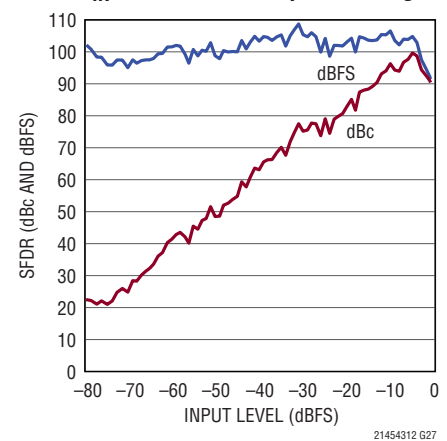
LTC2144-12: SFDR vs Input Level, f_{IN} = 70\text{MHz} , 105\text{Mps} , 2\text{V} Range
