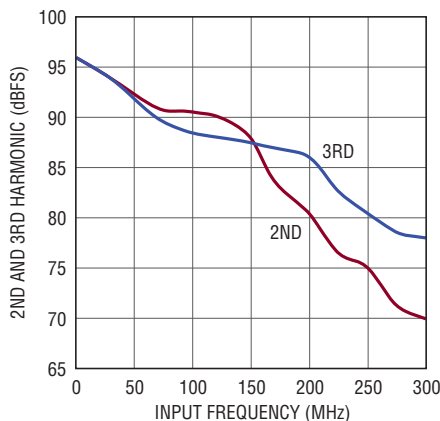
LTC2143-12: 2nd, 3rd Harmonic vs Input Frequency, -1\text{dBFS}, 80\text{Mps}, 2V Range
