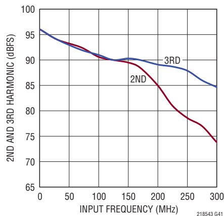
LTC2143-14: 2nd, 3rd Harmonic vs Input Frequency, -1dBFS, 80Mps, 1V Range
