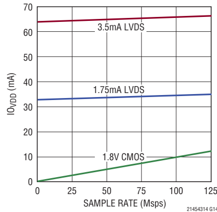
LTC2145-14: I_{O_{VDD}} vs Sample Rate, 5MHz, -1dBFS, Sine Wave on Each Input
