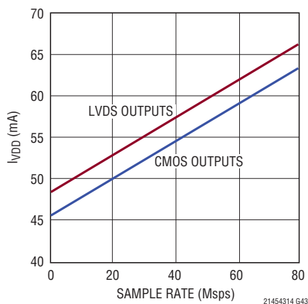
LTC2143-14: I_{VDD} vs Sample Rate, 5MHz, -1dBFS, Sine Wave Input on Each Channel
