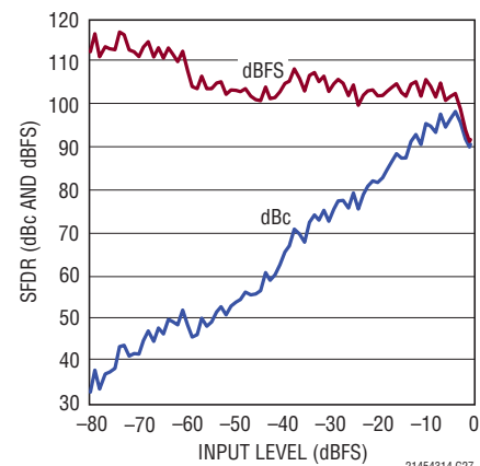
LTC2144-14: SFDR vs Input Level, f_{IN} = 70\text{MHz} , 105\text{Mps} , 2\text{V} Range
