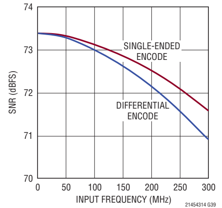
LTC2143-14: SNR vs Input Frequency, -1dBFS, 80Mps, 2V Range
