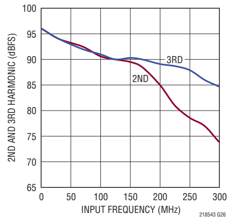
LTC2144-14: 2nd, 3rd Harmonic vs Input Frequency, -1\text{dBFS} , 105\text{Mps} , 1\text{V} Range
