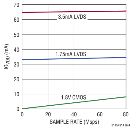
LTC2143-14: I_{O_{VDD}} vs Sample Rate, 5MHz, -1dBFS, Sine Wave Input on Each Channel
