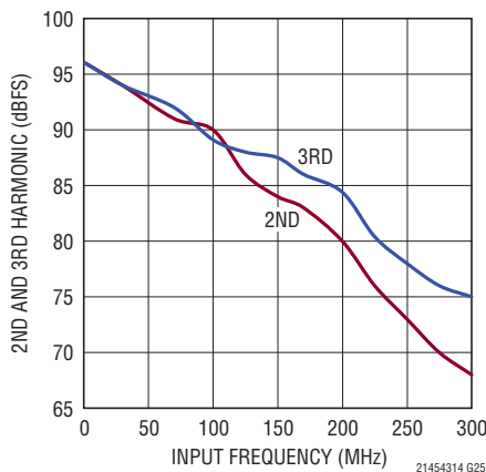
LTC2144-14: 2nd, 3rd Harmonic vs Input Frequency, -1\text{dBFS} , 105\text{Mps} , 2\text{V} Range
