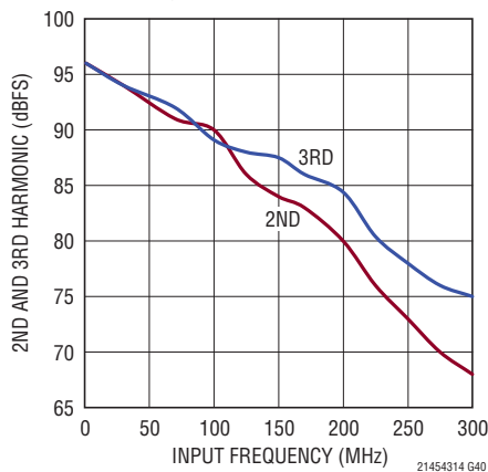
LTC2143-14: 2nd, 3rd Harmonic vs Input Frequency, -1dBFS, 80Mps, 2V Range
