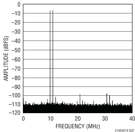
LTC2143-14: 64k Point 2-Tone FFT, f_{IN} = 69\text{MHz}, 70\text{MHz}, -1\text{dBFS}, 80Mps
