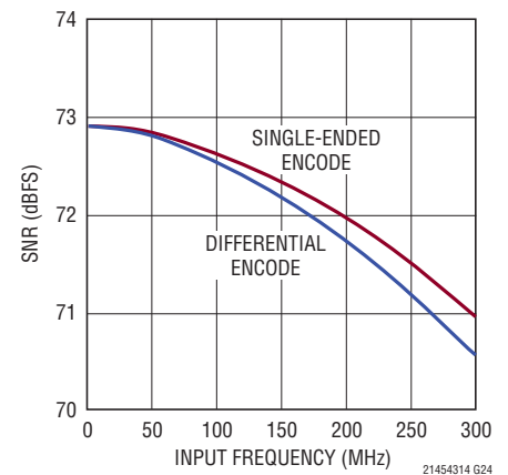
LTC2144-14: SNR vs Input Frequency, -1\text{dBFS} , 105\text{Mps} , 2\text{V} Range
