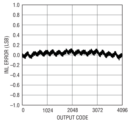
LTC2144-12: Integral Non-Linearity (INL)
