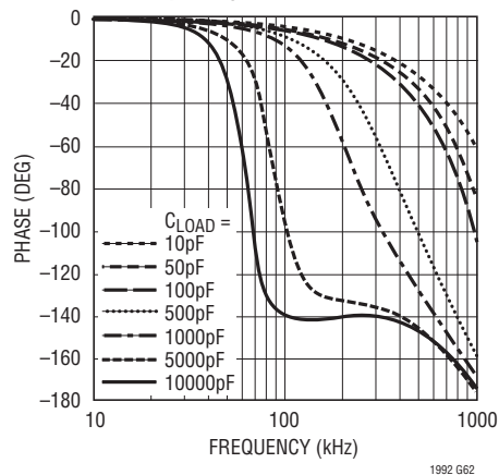
Differential Phase Response vs Frequency
