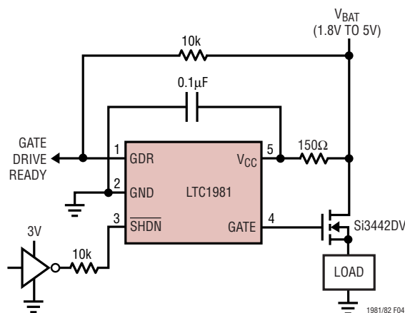
Figure 4. Reverse Battery Protection
