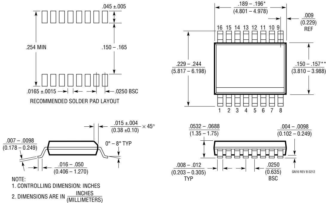
GN Package 16-Lead Plastic SSOP (Narrow .150 Inch) (Reference LTC DWG # 05-08-1641 Rev B)
