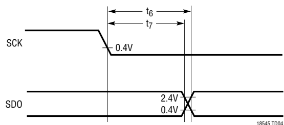
t_6 (Delay Time, \overline{SCK} \downarrow to SDO Valid) t_7 (Time from Previous Data Remains Valid After \overline{SCK} \downarrow )
