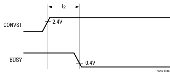
t_2 (CONVST to \overline{BUSY} Delay)
