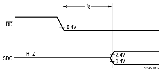
t_8 (SDO Valid After \overline{RD} \downarrow )
