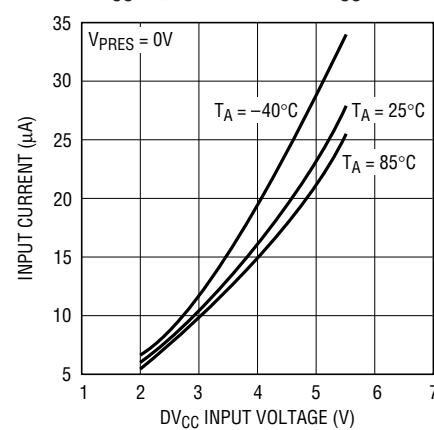
DV_{CC} Input Current vs DV_{CC} Voltage
