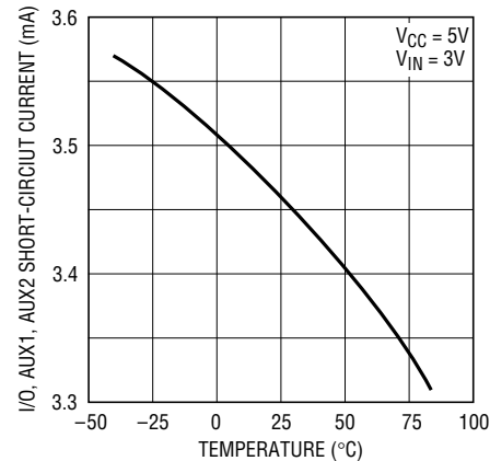
I/O, AUX1, AUX2 Short-Circuit Current vs Temperature
