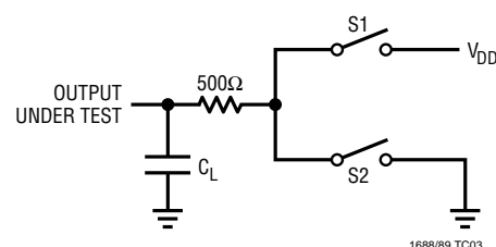
Figure 3. Driver Timing Test Load
