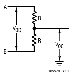
Figure 1. Driver DC Test Load
