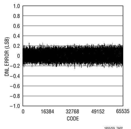
Differential Nonlinearity vs Input Code
