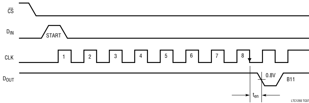
Voltage Waveforms for t_{en}
