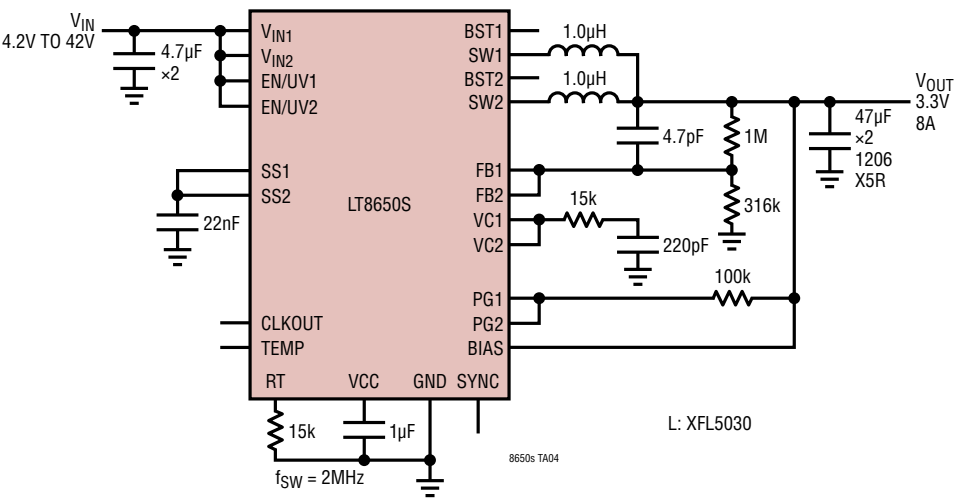
Two Phase, 3.3V, 8A, 2MHz Step-Down Converter
