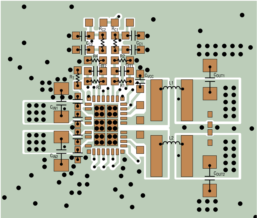
Figure 9. Recommended Layout
