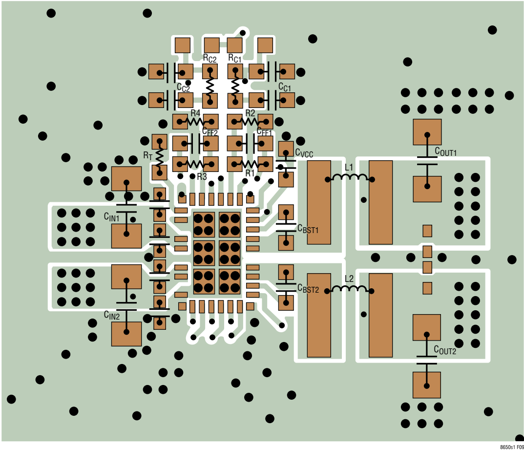
Figure 9. Recommended Layout
