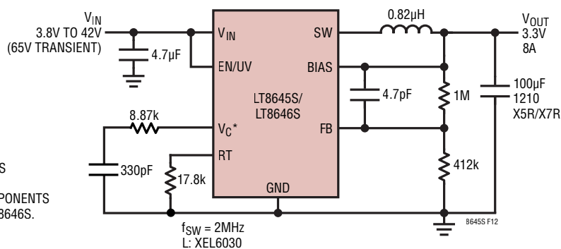
Figure 12. 2MHz 3.3V, 8A Step-Down Converter
